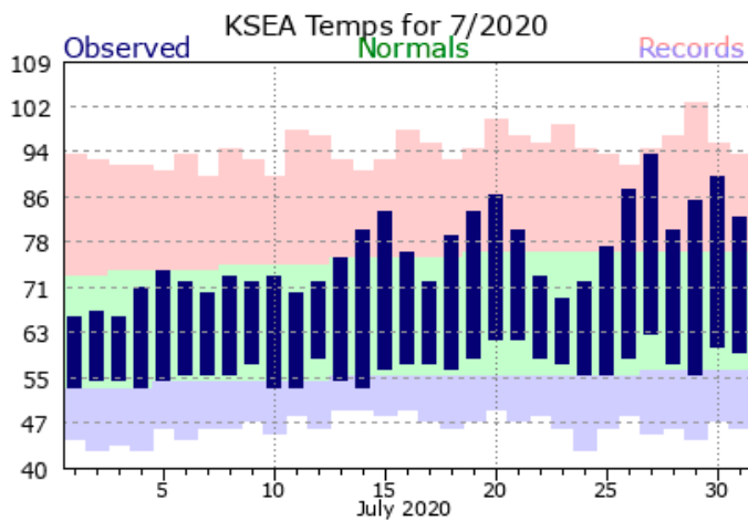
Figure 2: Daily July 2020 maximum and minimum temperatures compared to normal (green envelope) and records (red and blue bars) for (a) SeaTac Airport and (b) Pasco (NWS).
