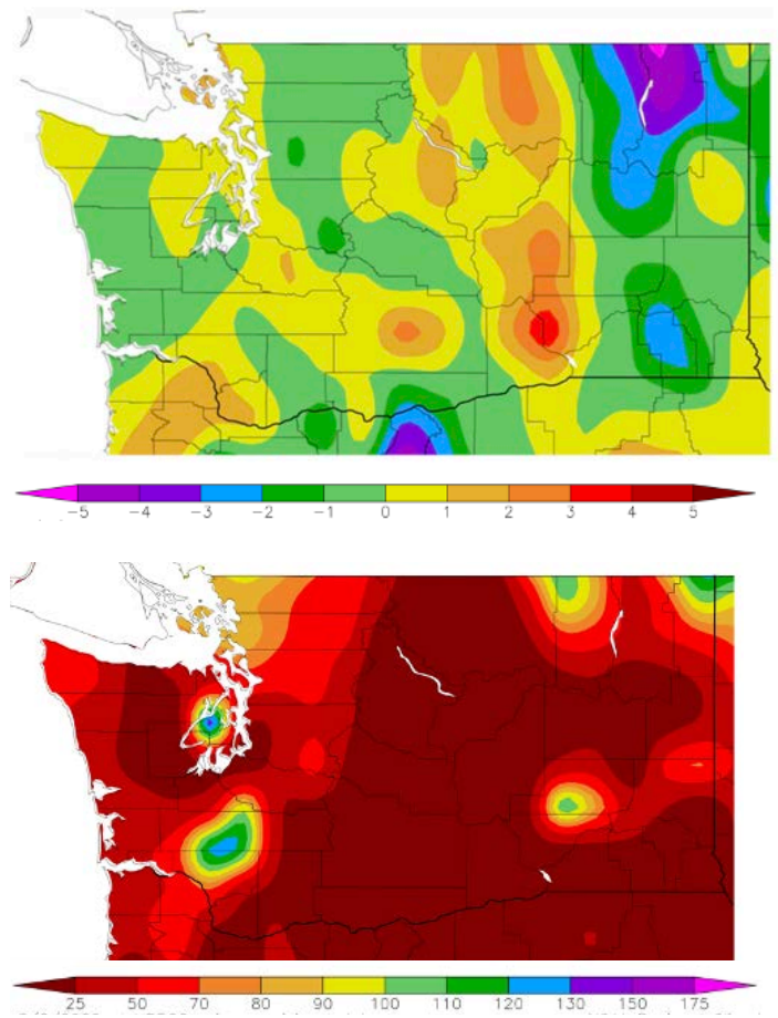
Figure 9: July temperature (°F) departure from normal (top) and precipitation percent of normal (bottom). ( High Plains Regional Climate Center ; relative to the 1981-2010 normal).
