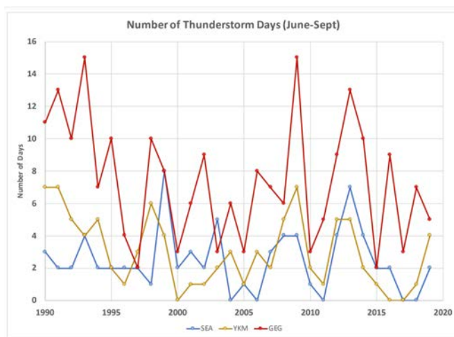
Figure 7: Thunderstorm days during June through September in Seattle (KSEA; blue trace), in Yakima (KYKM; gold trace) and Spokane (KGEG; red trace) for the years of 1990-2019.
