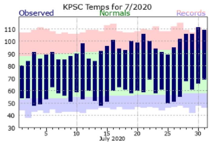
Figure 2: Daily July 2020 maximum and minimum temperatures compared to normal (green envelope) and records (red and blue bars) for (a) SeaTac Airport and (b) Pasco (NWS).
