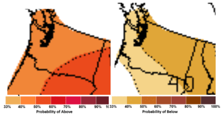
Figure 10: August outlook for temperature (left) and precipitation (right) ( Climate Prediction Center ).
