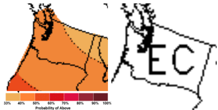
Figure 11: August outlook for temperature (left) and precipitation (right) ( Climate Prediction Center ).
