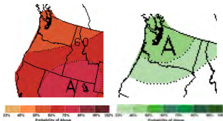
October outlook for temperature (left) and precipitation (right)
