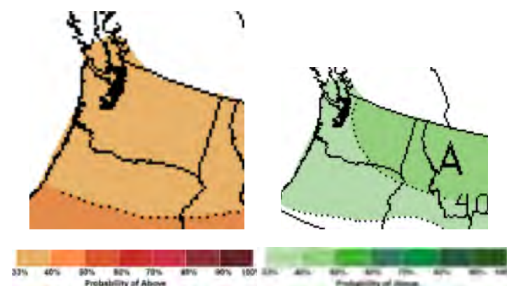
October-November-December outlook for temperature (left) and precipitation (right)
