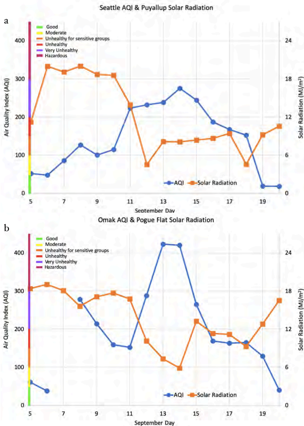
Figure 6: Daily average AQI for (a) Seattle and (b) Omak with daily solar radiation from nearby Puyallup (a) and Pogue Flat (b) WSU's AgWeatherNetwork (AWN) stations for 5-20 September 2020.
