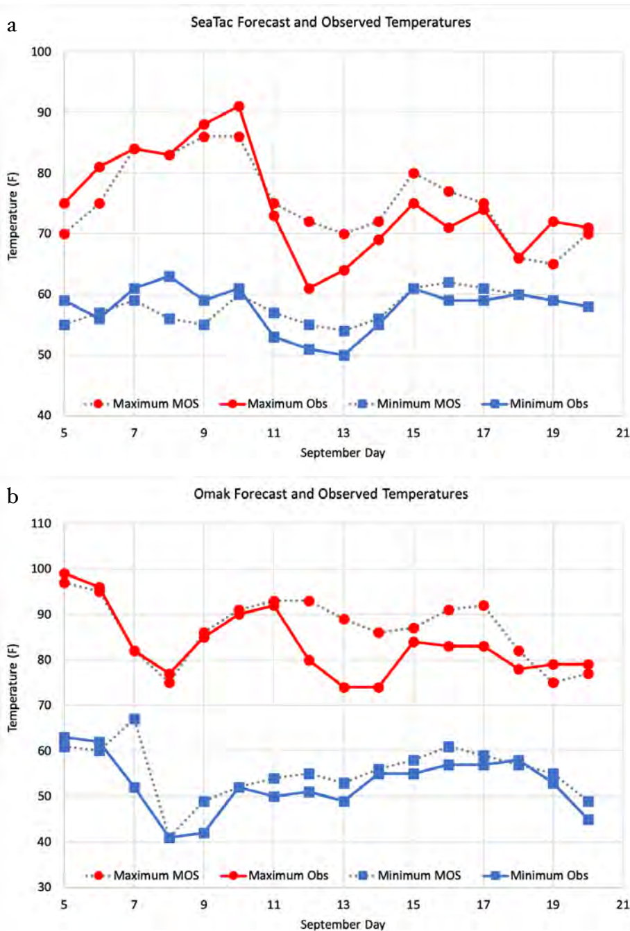
Figure 7: Time series of GFS maximum and minimum temperature forecasts and corresponding observed temperatures for (a) SeaTac Airport (KSEA) and (b) Omak (KOMK) for 5-20 September 2020.
