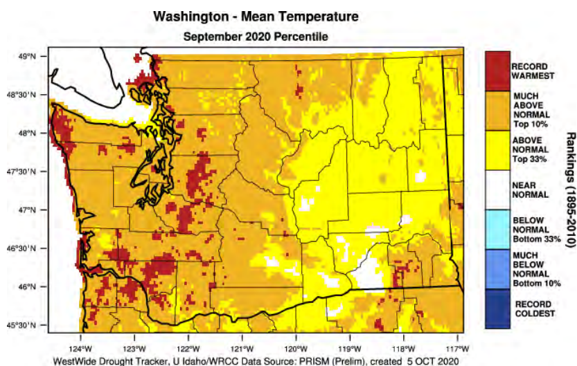
Figure 1: September 2020 mean temperature percentiles (using the 1895-2010 baseline) from WWDt .
