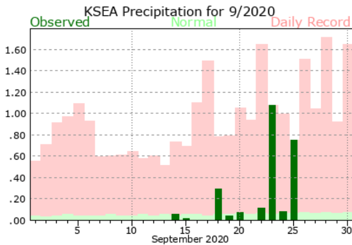
Figure 2: Daily September 2020 precipitation for SeaTac Airport ( NWS ).
