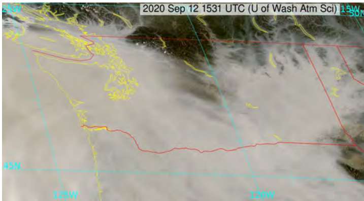
Figure 5: Visible satellite image of smoke from 8:30 am on 12 September.
