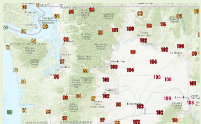
Figure 8: Maximum temperatures on August 16th from NWS .
