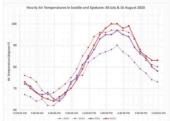
Figure 11: Hourly air temperatures (degrees F) for Seattle (KSEA; purple) and Spokane (KGEG; crimson) during 30 July (dotted lines) and 16 August (solid lines) of 2020. Times are in Pacific Daylight Time (PDT).
