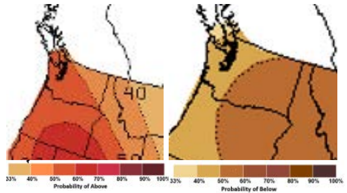
Figure 13: September outlook for temperature (left) and precipitation (right).
