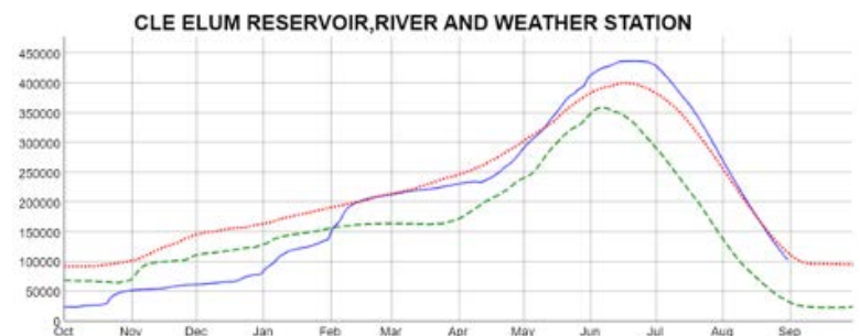
Figure 5: Water year summary of the Cle Elum Reservoir, the largest reservoir in the Yakima basin. Red is the mean storage, blue is current water year 2020, and green is water year 2019 ( from Bureau of Reclamation ).
