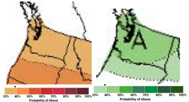
Figure 14: September-October-November outlook for temperature (left) and precipitation (right) ( Climate Prediction Center ).
