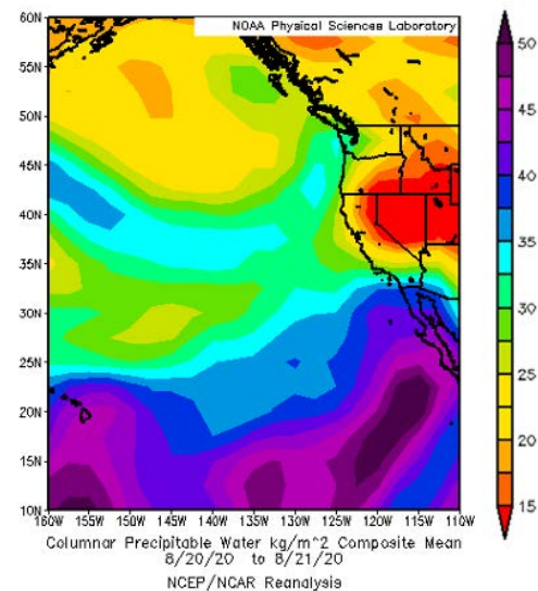
Figure 2: Precipitable water reanalysis between 1000 - 500 hPa (~18,000 feet) from NCEP .
