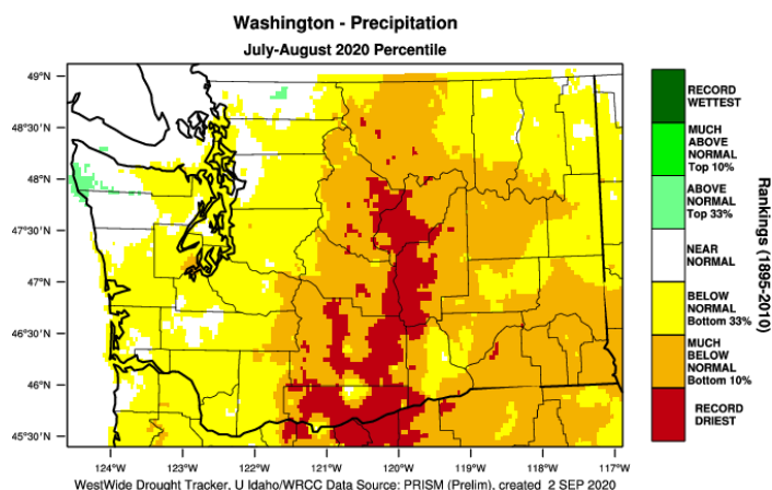
Figure 1a (left) shows the percentile ranking of precipitation for July and August. Figure 1b (right) is the same metric except for the meteorological summer, June through August (from Westwide Drought Tracker ).
