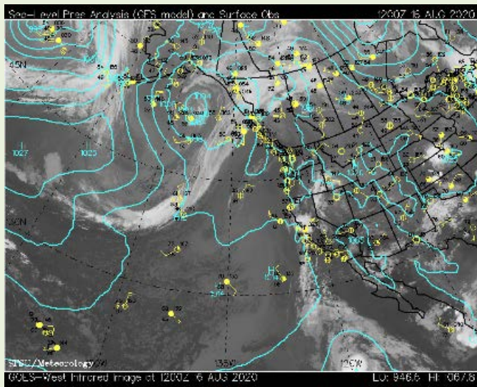
Figure 9: GOES-West 17 infrared satellite imagery of North America with surface pressure model analysis ( California Regional Weather Server ).
