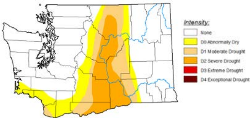
Figure 3: The August 2020 edition of the U.S. Drought Monitor .
