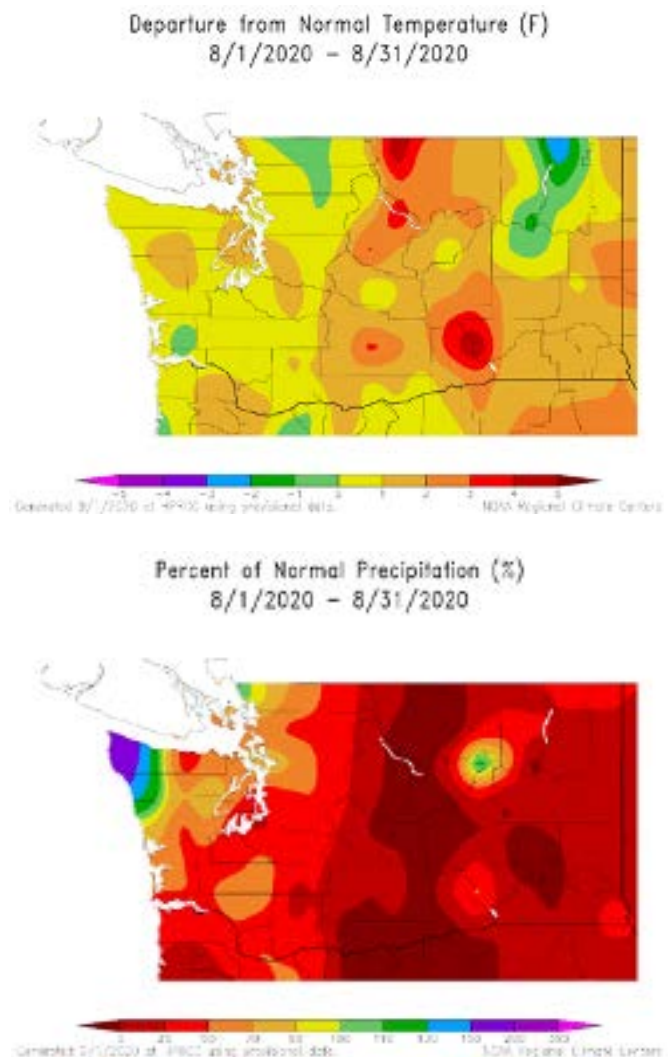
Figure 12: August temperature (°F) departure from normal (top) and precipitation percent of normal (bottom). ( High Plains Regional Climate Center ; relative to the 1981-2010 normal).
