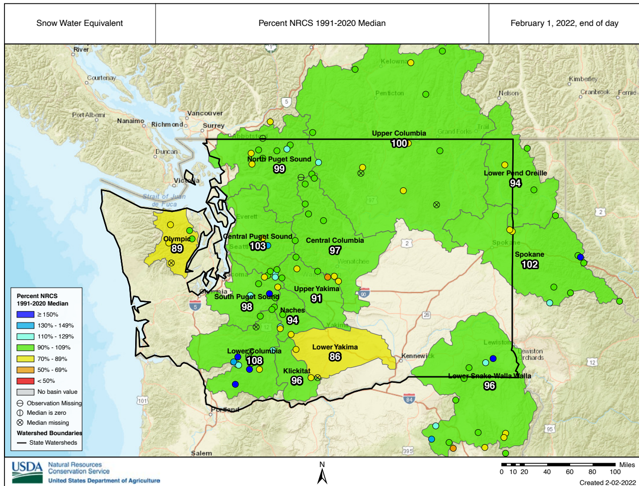
Figure 3: Snowpack (in terms of snow water equivalent) percent of median for WA as of February 1, 2022. The median is based on the 1991-2020 period (NRCS).
