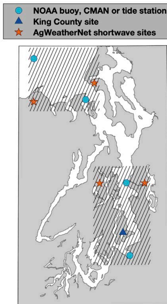
Figure 5: The locations of the “North Sound” and “Central Sound” regions (hatched areas) and the observations used to calculate the fluxes ( Puget Sound Metrics Dashboard ).
