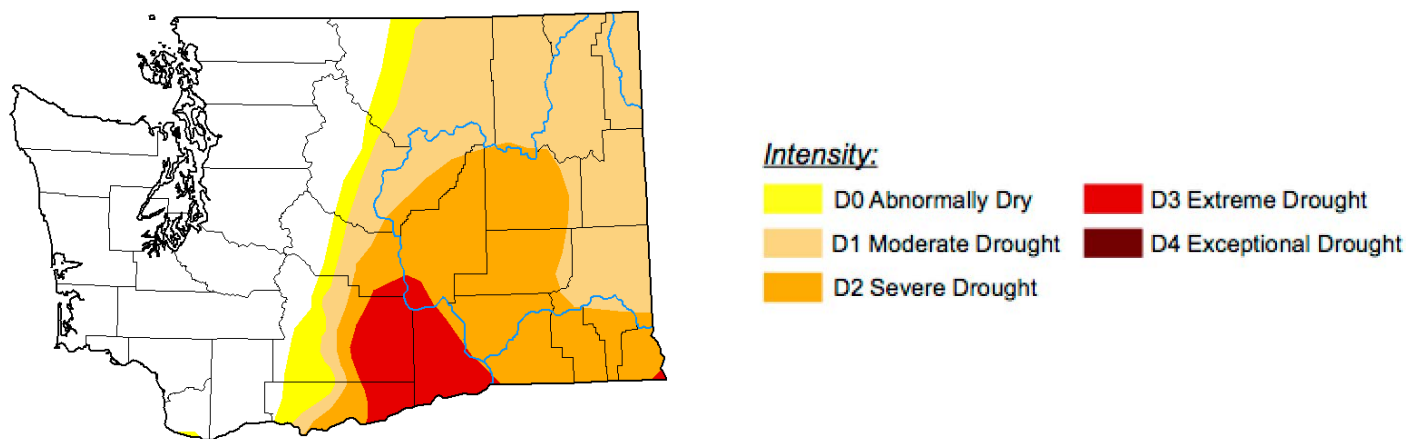
Figure 4: The February 3, 2022 edition of the U.S. Drought Monitor .
