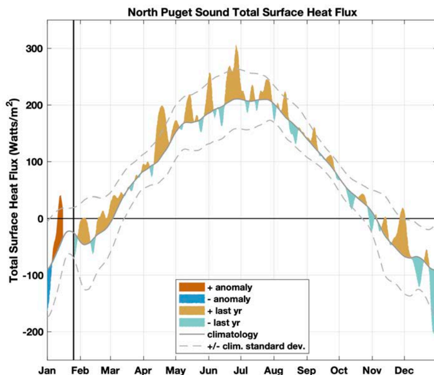
Figure 6: February 2021-January 2022 total surface heat flux for the North Puget Sound region compared to a 7-year climatology ( Puget Sound Metrics Dashboard ).
