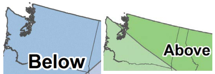
Figure 9: February-March-April outlook for temperature (left) and precipitation (right) (Climate Prediction Center).
