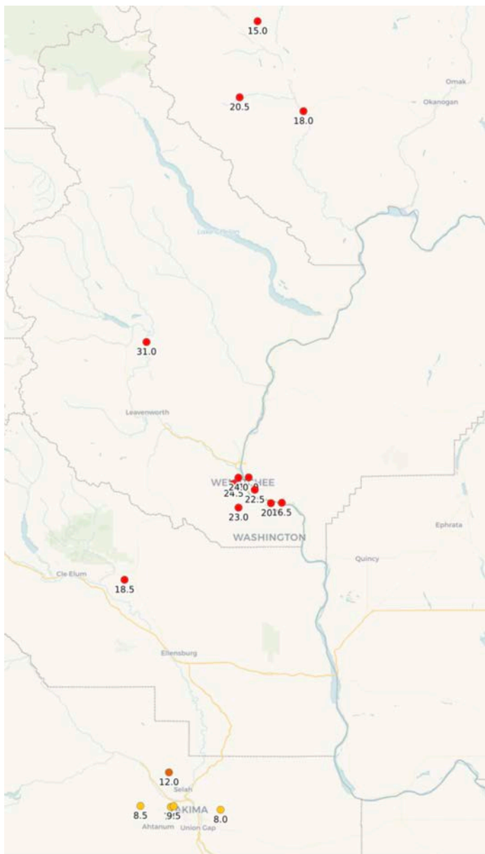
Figure 2: 24-hour snowfall measurements on the morning of January 6, 2022 from the CoCoRaHS network.
