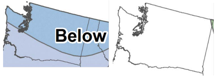
Figure 8: February outlook for temperature (left) and precipitation (right).
