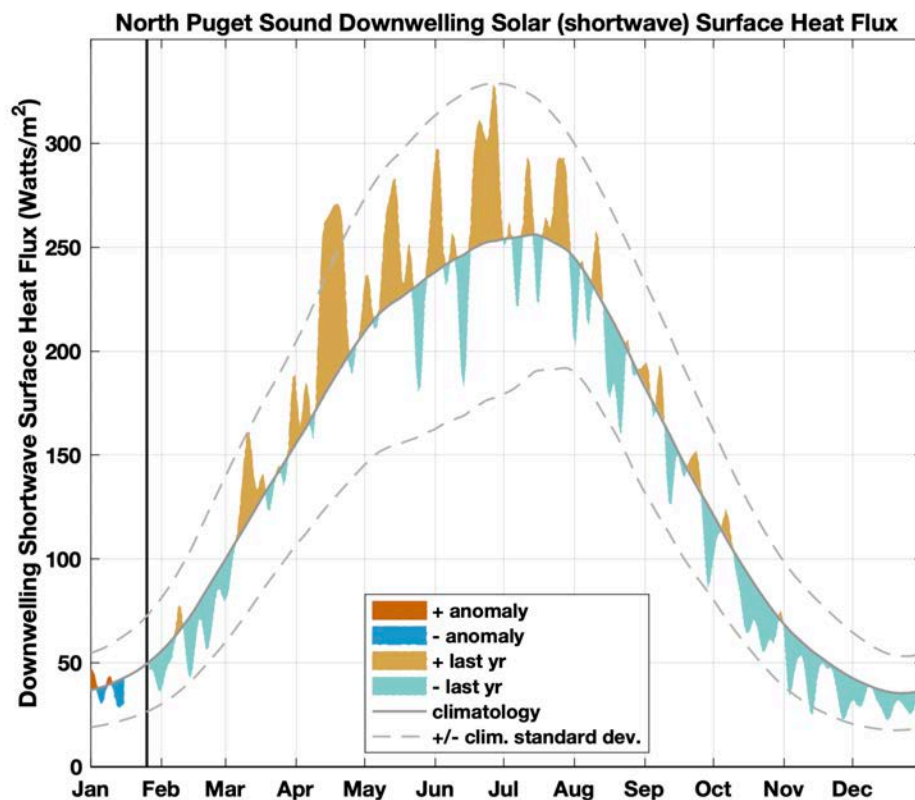
Figure 7: February 2021-January 2022 downwelling solar surface heat flux for the North Puget Sound region compared to a 7-year climatology ( Puget Sound Metrics Dashboard ).
