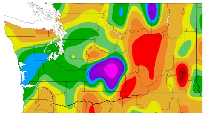
Precipitation (%)
