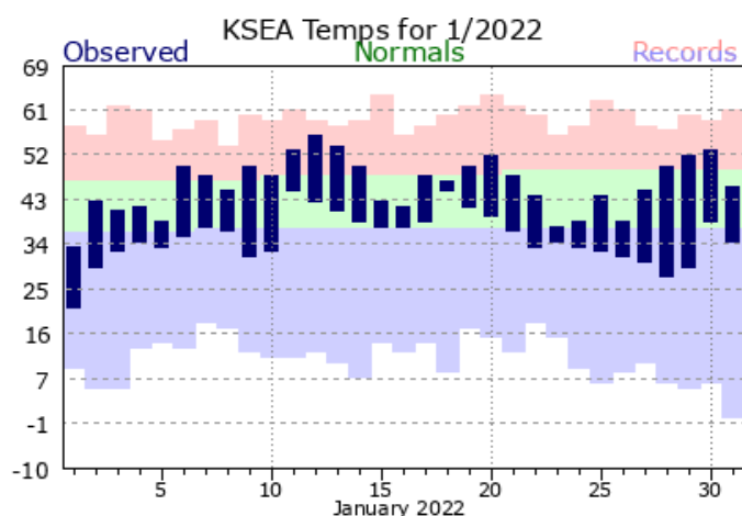
Figure 1: January 2022 daily temperature and precipitation for Sea-Tac Airport compared to the 1991-2020 normal (green envelope) and previous records (blue and red envelopes; NWS ).
