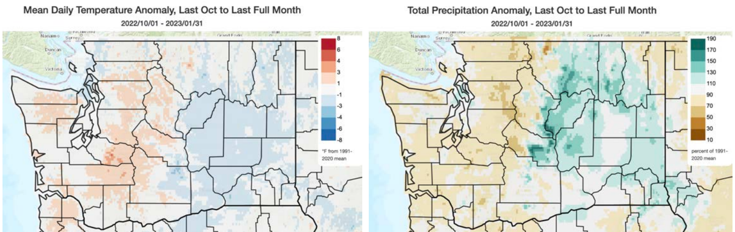
Figure 1: October 2022-January 2023 average temperature departure from the 1991-2020 normal (left) and total precipitation percent of normal (right) from Climate Toolbox .
