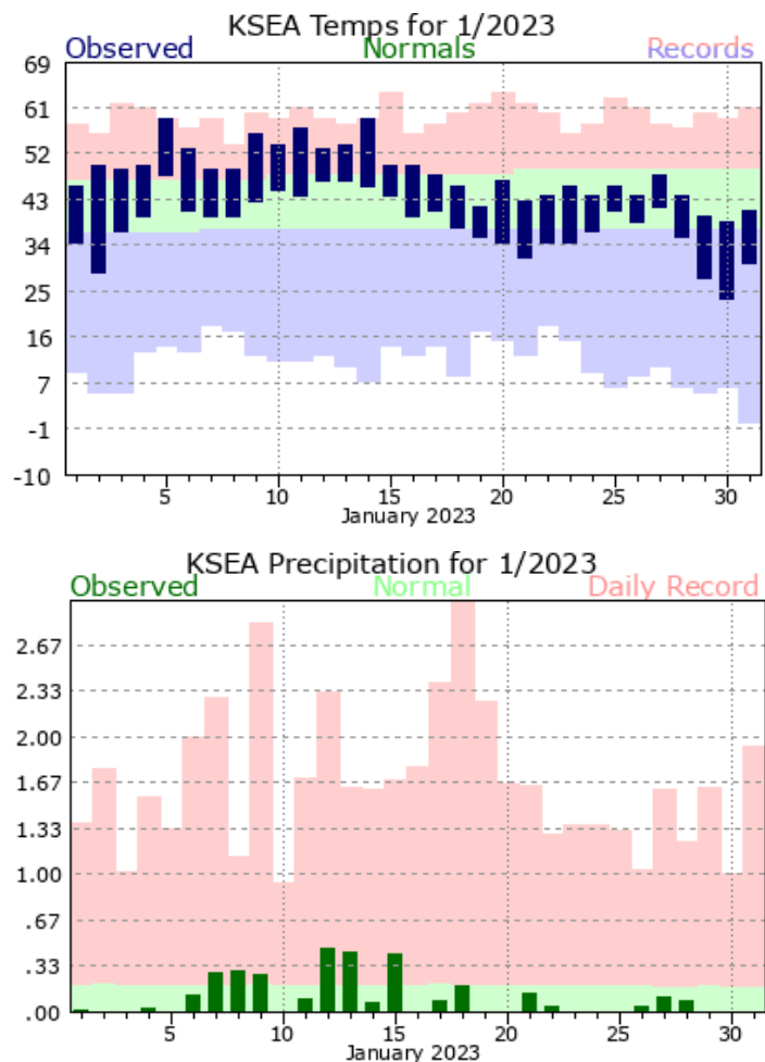
Figure 2: January 2023 daily temperatures for SeaTac Airport compared to the 1991-2020 normal (green envelope) and previous records (blue and red envelopes; NWS ).
