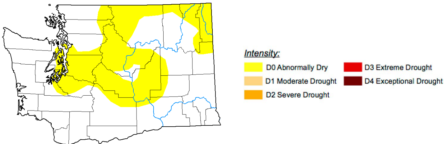
Figure 4: The February 2, 2023 edition of the U.S. Drought Monitor .
