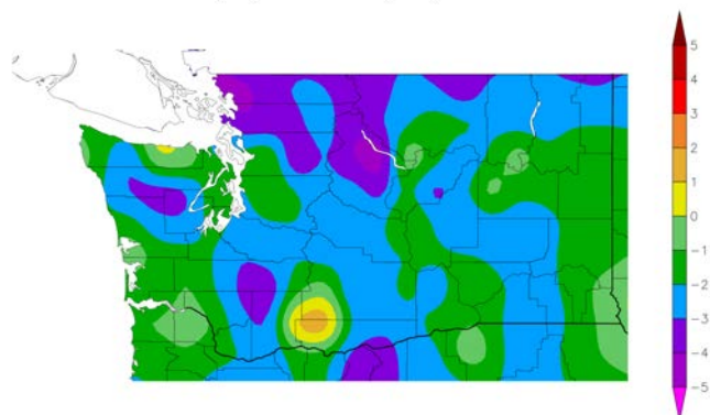
Departure from Normal Temperature (F) 4/1/2023 - 4/30/2023
