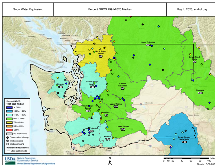
Figure 3: Snowpack (in terms of snow water equivalent) percent of normal for Washington as of May 1, 2023 (NRCS).
