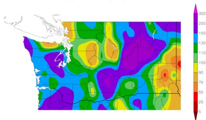
Percent of Normal Precipitation (%) 4/1/2023 - 4/30/2023
