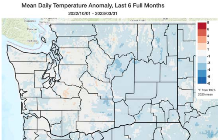
Figure 7: October 2022 through March 2023 (a) average temperature departure from the 1991-2020 normal and (b) precipitation percent of normal for WA state (from Climate Toolbox ).
