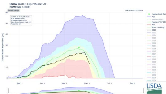
Figure 4: 2023 water year snow water equivalent (black trace) compared to median (green trace) and prior years, including the maximum (blue trace) and minimum (red trace), at the Bumping Ridge Snotel site in the Naches Basin (NRCS).
