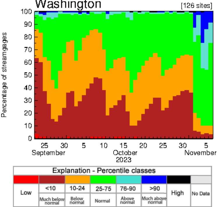
Figure 5: The percentage of stream gauges in WA in each percentile category from late September through early November (USGS).
