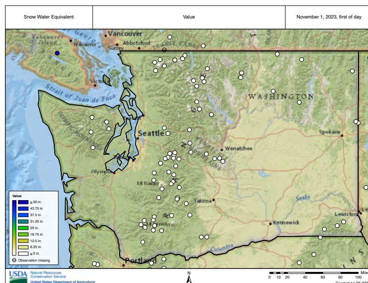
Figure 3: The snow water equivalent value (in inches) as of November 1, 2023. White circles represent no snow (NRCS).
