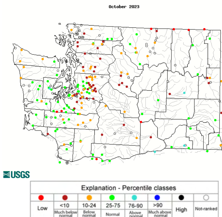
Figure 4: October 2023 average streamflow percentiles (USGS).
