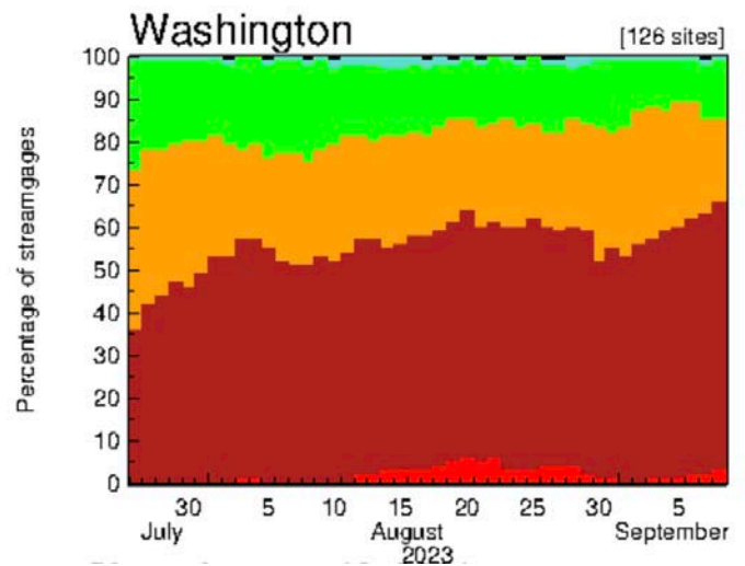
Figure 4: The percentage of stream gauges in WA in each percentile category shown in Figure 3 from late July through early September (USGS).
