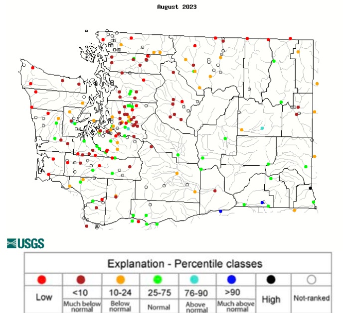
Figure 3: August 2023 average streamflow (USGS).
