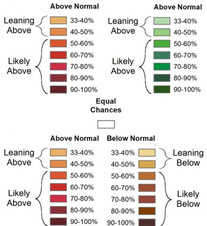
Figure 9: September outlook for temperature (left) and precipitation (right).
