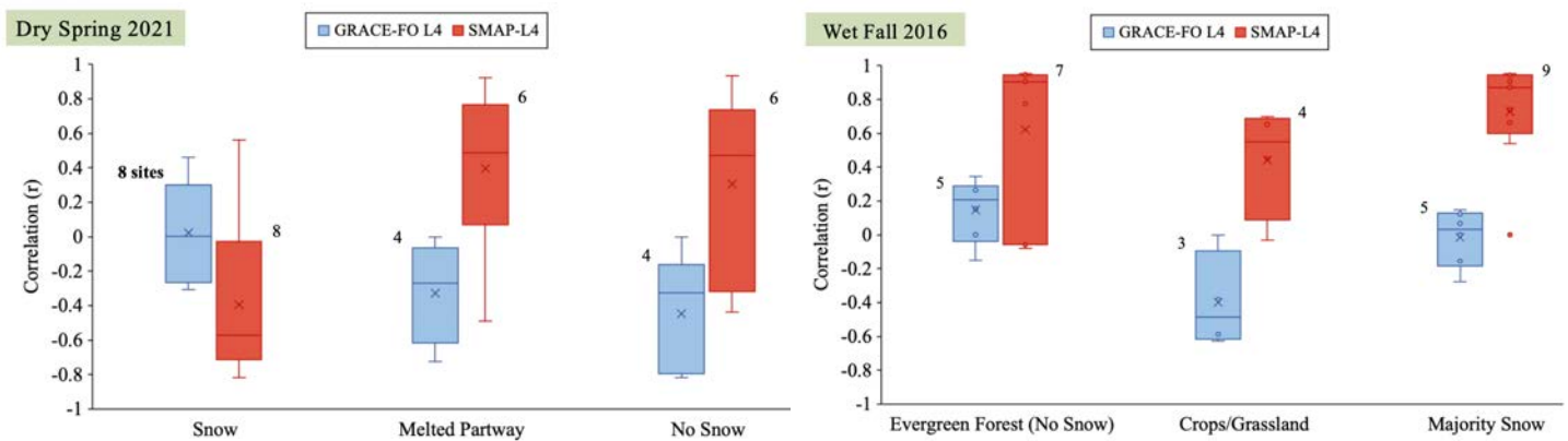
Figure 8: Pearson correlations between satellite-derived products and in situ observations.
