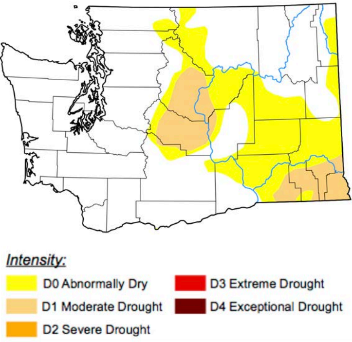
Figure 6: The December 5th, 2024 edition of the US Drought Monitor .
