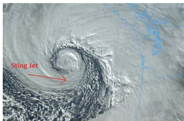
Figure 1: Bomb Cyclone off the coast of Washington on November 20, 2024 from NWS Seattle.
