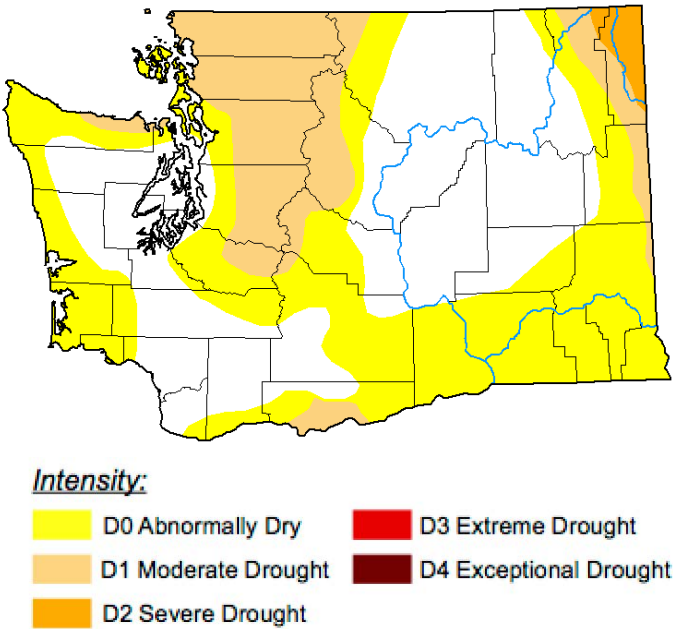
Figure 7: The January 2, 2024 edition of the U.S. Drought Monitor .
