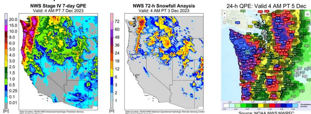
Figure 3: Observed 7-day precipitation, 72-hour snowfall, and 24-hour precipitation for different time periods during early December from CW3E Summary.
