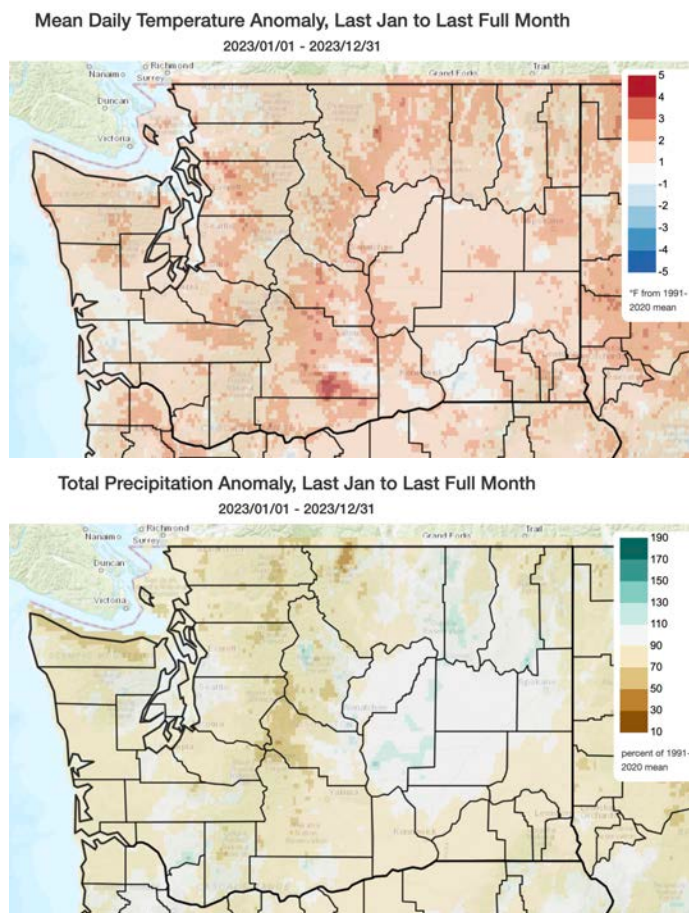
Figure 4: 2023 mean temperature anomalies (top) and precipitation percent of normal compared to the 1991-2020 period (Climate Toolbox).
