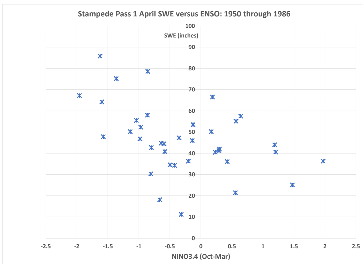
Figure 9: April 1 snow water equivalent (SWE) in inches at Stampede Pass (y-axis) vs. the October-March NINO 3.4 index (x-axis) for 1950 through 1986. Positive NINO 3.4 indices represent El Niño-like conditions: roughly between 0.5 and 1 are weak, 1 and 1.5 are moderate, and above 1.5 is strong. This scaling applies to the La Niña conditions as well, except those numbers are negative.
