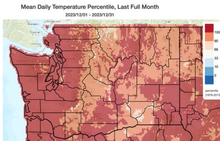
Figure 1: December 2023 temperature percentiles compared to the 1979-2015 record (Climate Toolbox).
